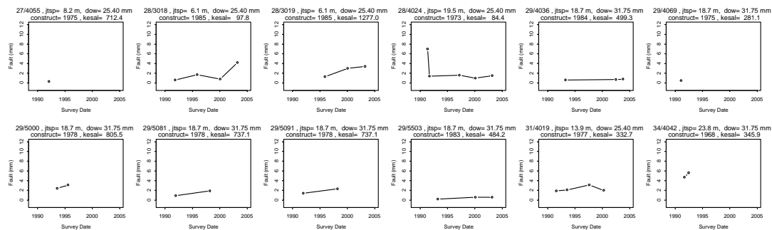
FIGURE 1 Faulting history of some dowelled jointed pavements.
