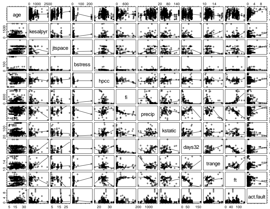
FIGURE 3 Scatter plot smoother and matrix for dowelled jointed pavements.
