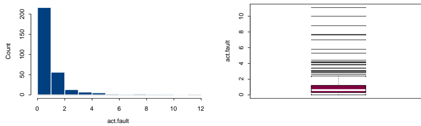
FIGURE 2 Exploratory data analysis: dowelled joint faulting.
