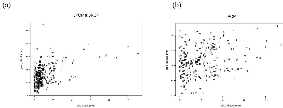
FIGURE 5 Goodness of prediction using 1998 AASHTO (a) dowelled; (b) nondowelled models.
