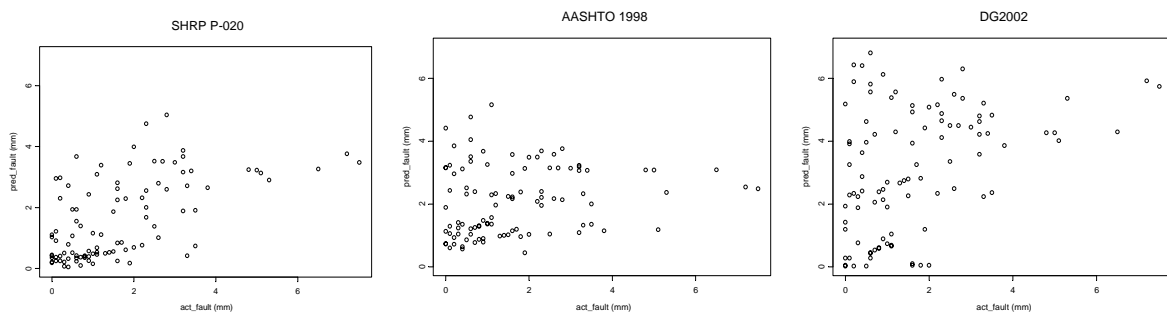
FIGURE 6 Goodness of prediction using (a) P-020; (b) 1998 AASHTO; and (c) DG2002 models.
