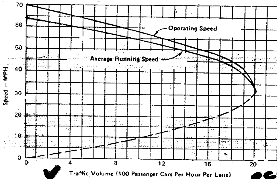
Figure II-23. Speed-volume relationship on six-lane freeways.
