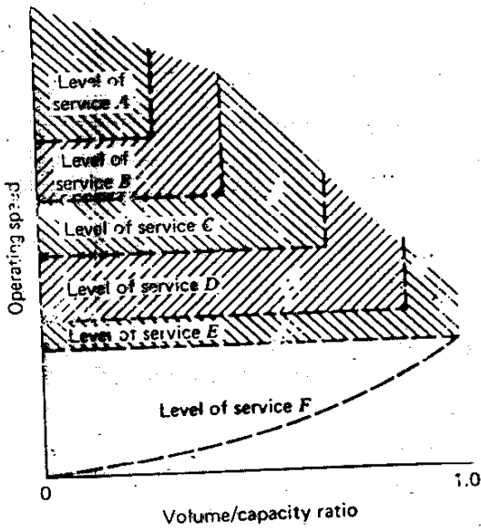
Fig 4-10. General concept of relationship of level of service to operating speed and volume/capacity ratio (not to scale). (Courtesy Transportation Research Board.)
