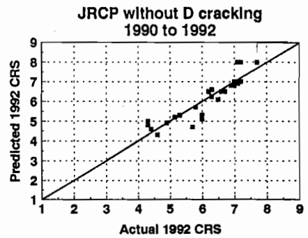
FIGURE 2 Predicted versus actual 1992 CRS for JRCR without D-cracking.
