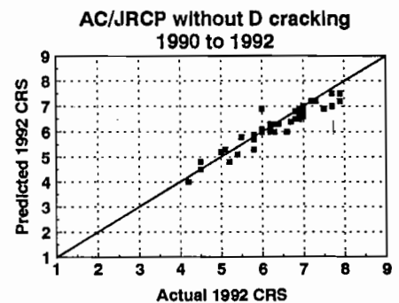
FIGURE 4 Predicted versus actual 1992 CRS for AC-overlaid JRCR without D-cracking.
