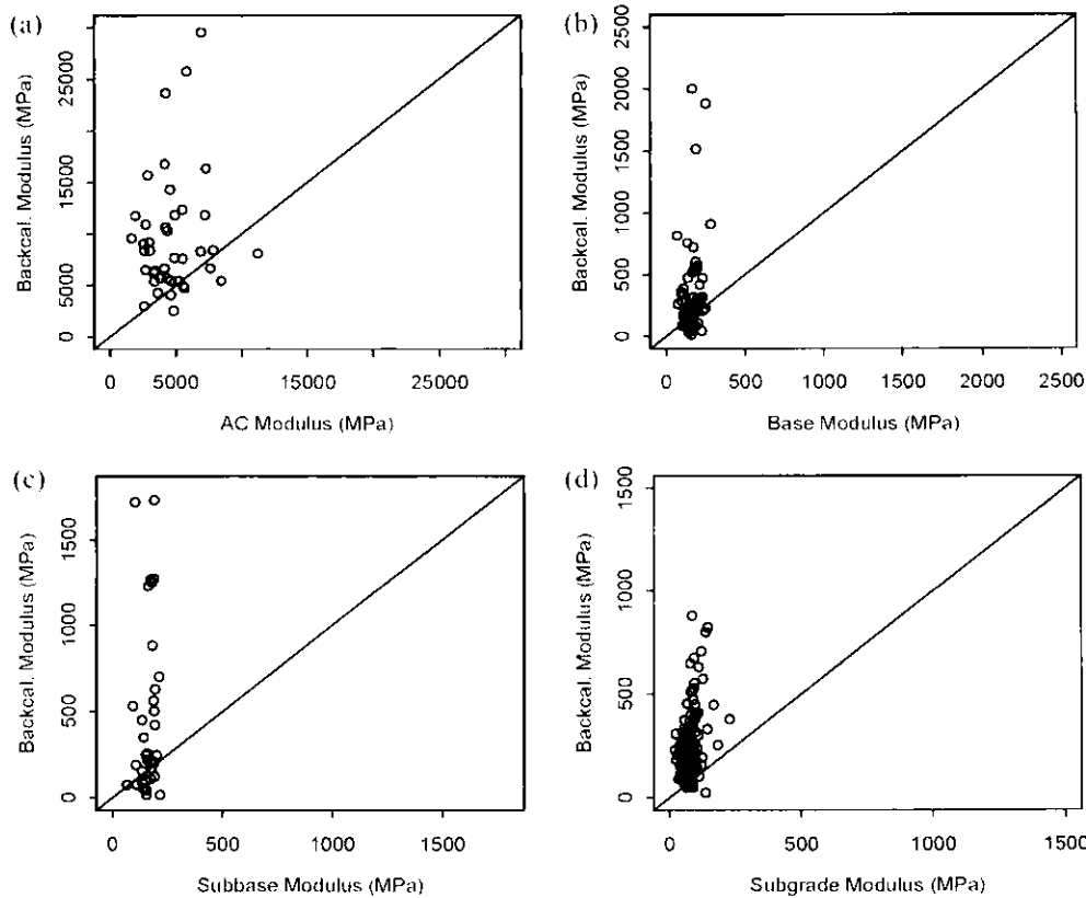
Figure 3. Comparison of layer moduli of (a) AC surface layer; (b) base layer; (c) subbase layer; and (d) subgrade obtained from laboratory testing and backcalculation program.
