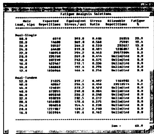
Figure 3. Sample fatigue analysis output screen
