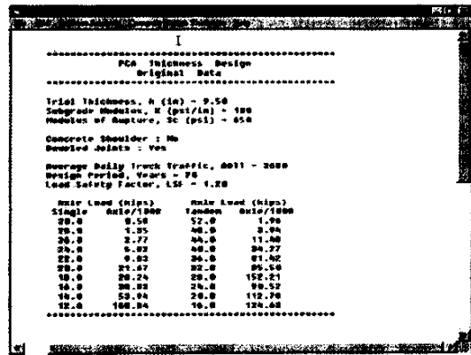
Figure 2. Sample output screen of the design inputs
