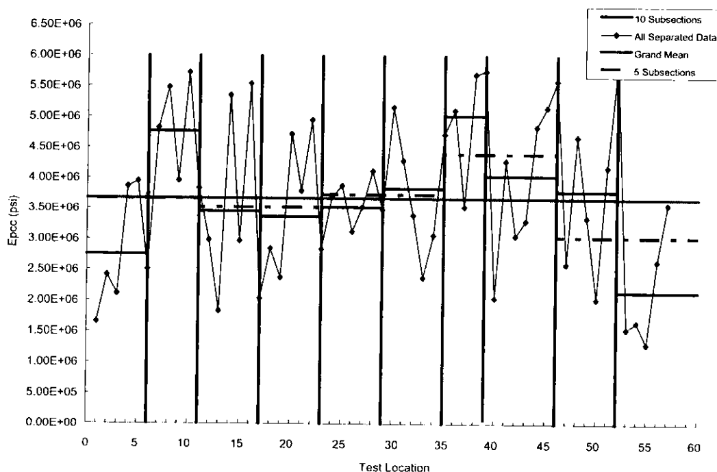
Figure 3. Variation of the backcalculated moduli of the slab.
