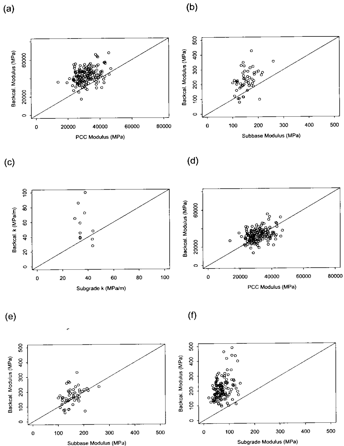
Figure 1. Comparison of laboratory tested and backcalculated layer moduli of: (a) surface, (b) subbase, and (c) subgrade for dense liquid foundation; and (d), (e), (f) for elastic solid foundation, respectively.
