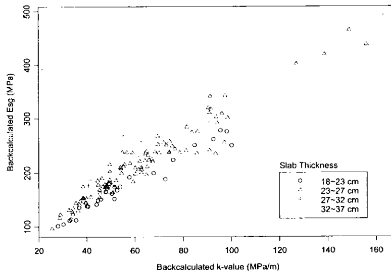
Figure 2. Comparison of elastic solid foundation versus dense liquid foundation based on backcalculated results.
