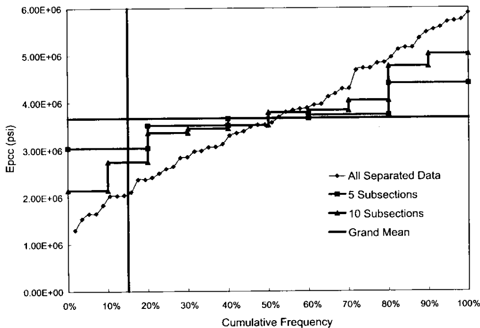
Figure 4. Cumulative frequency of different evaluation methods (Note: 1 psi = 6.89 kPa).
