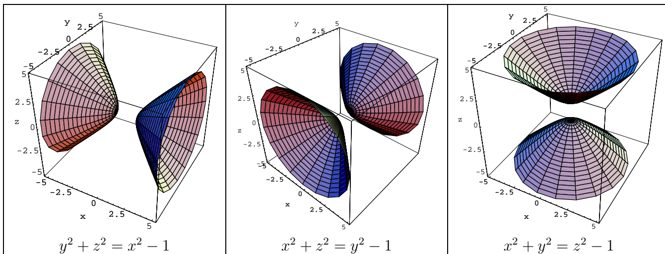
Hyperboloids of two sheets
