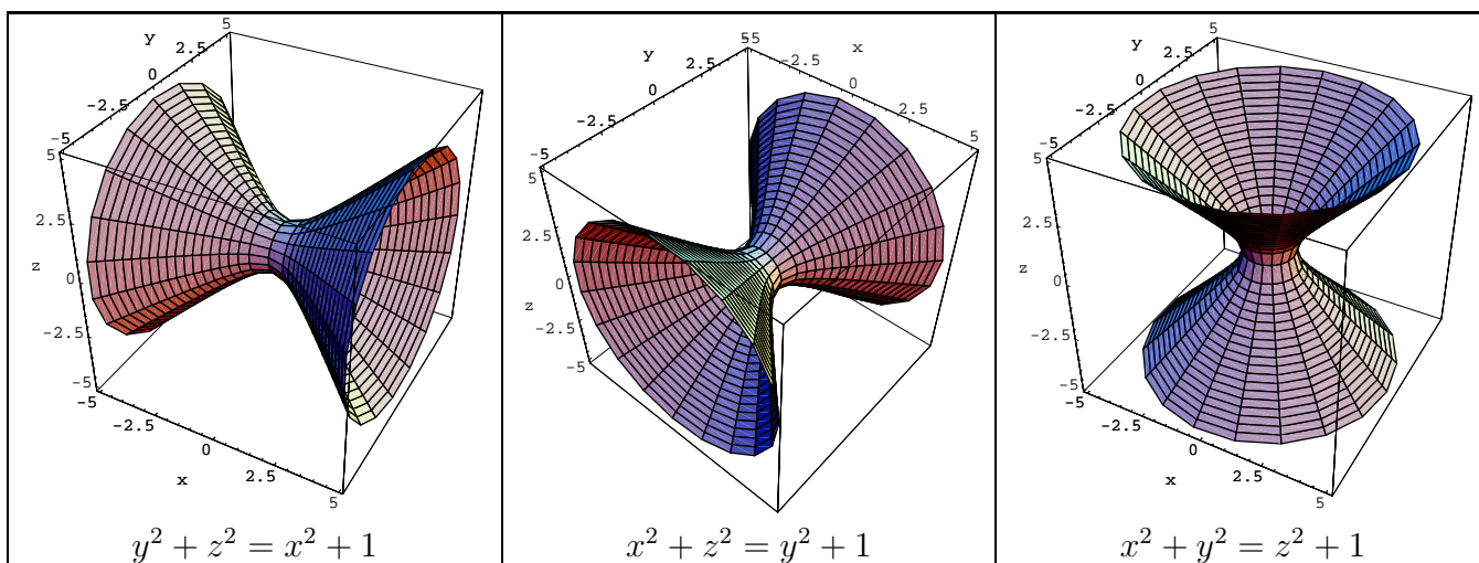
Hyperboloids of one sheet
